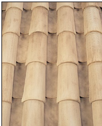
B319-R Ivory Smoke Blend Solar Reflectance Avg. - 0.43 Thermal Emittance Avg. - 0.82
