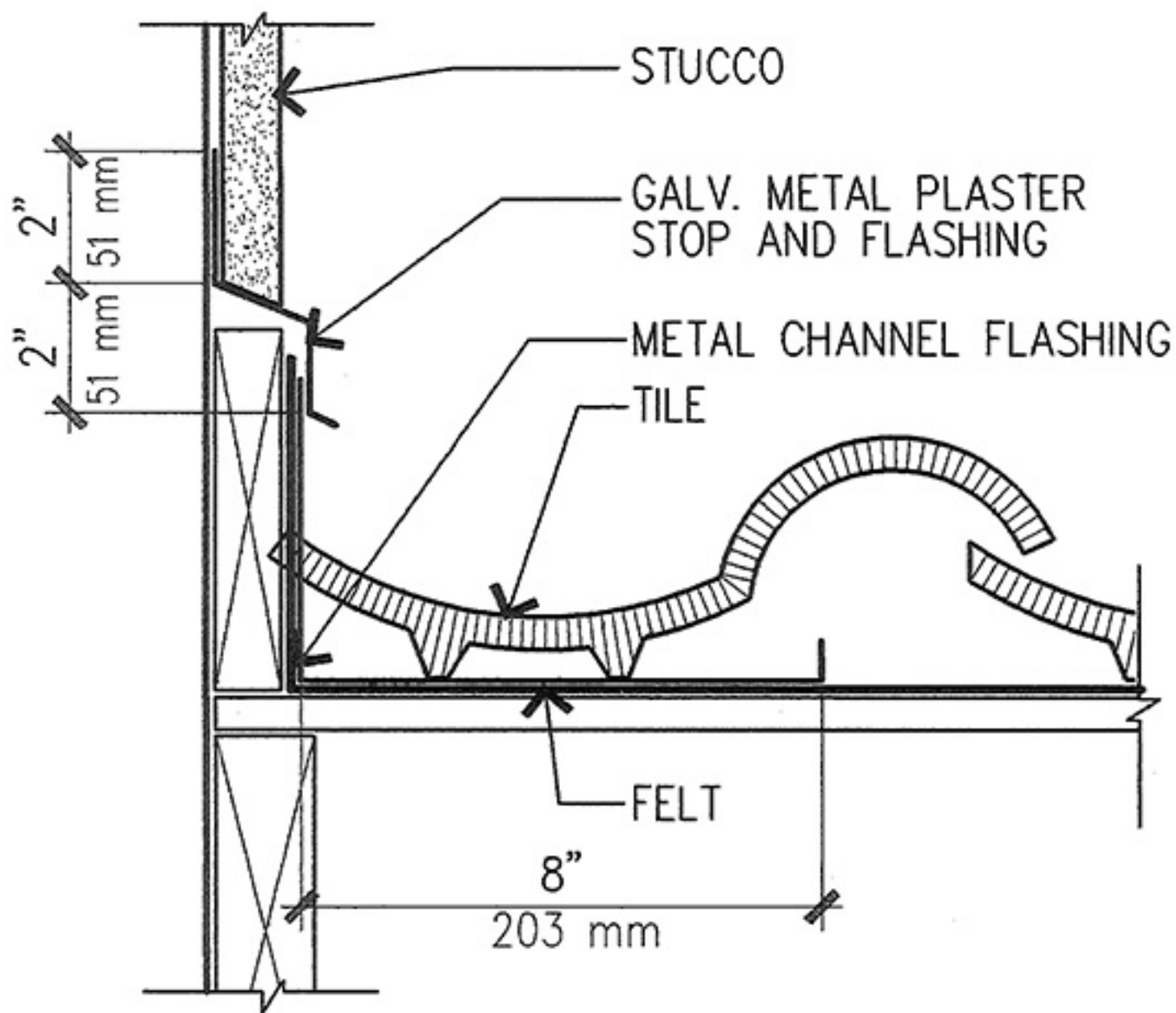
FLASHING DETAIL AT WALL
