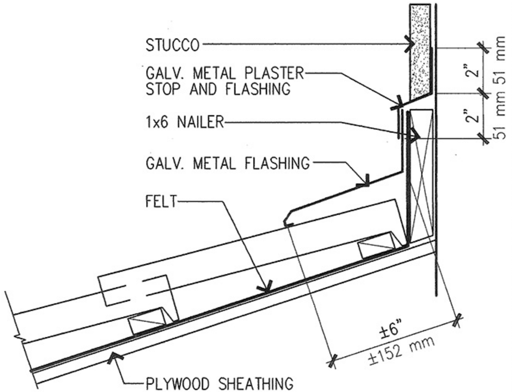
FLASHING DETAIL AT WALL
