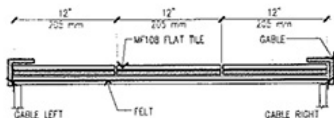
SPACE DETAIL
