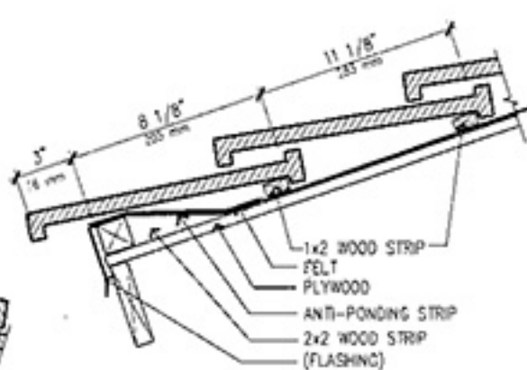
EAVE DETAIL
