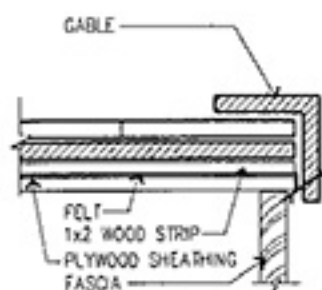
GABLE DETAIL
