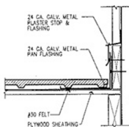
FLASHING DETAIL AT WALL
