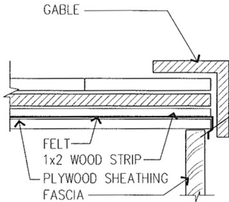
GABLE DETAIL
