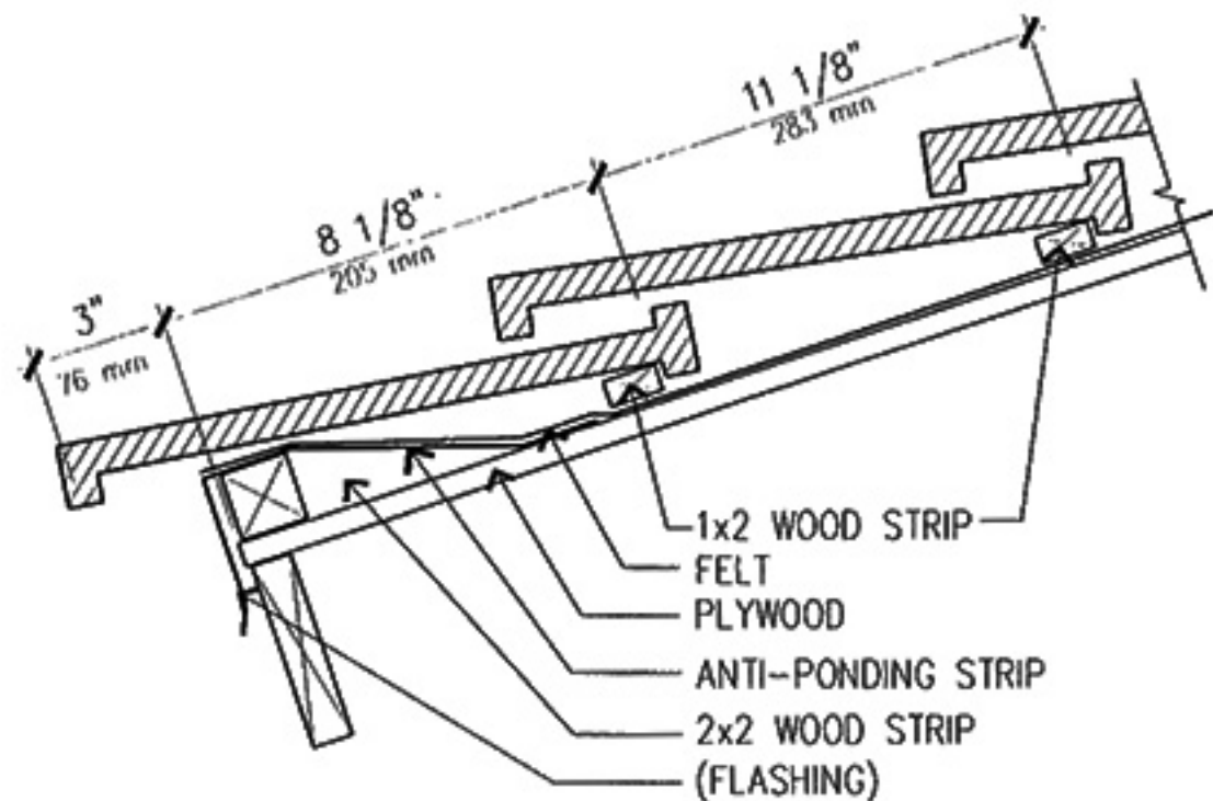
EAVE DETAIL
