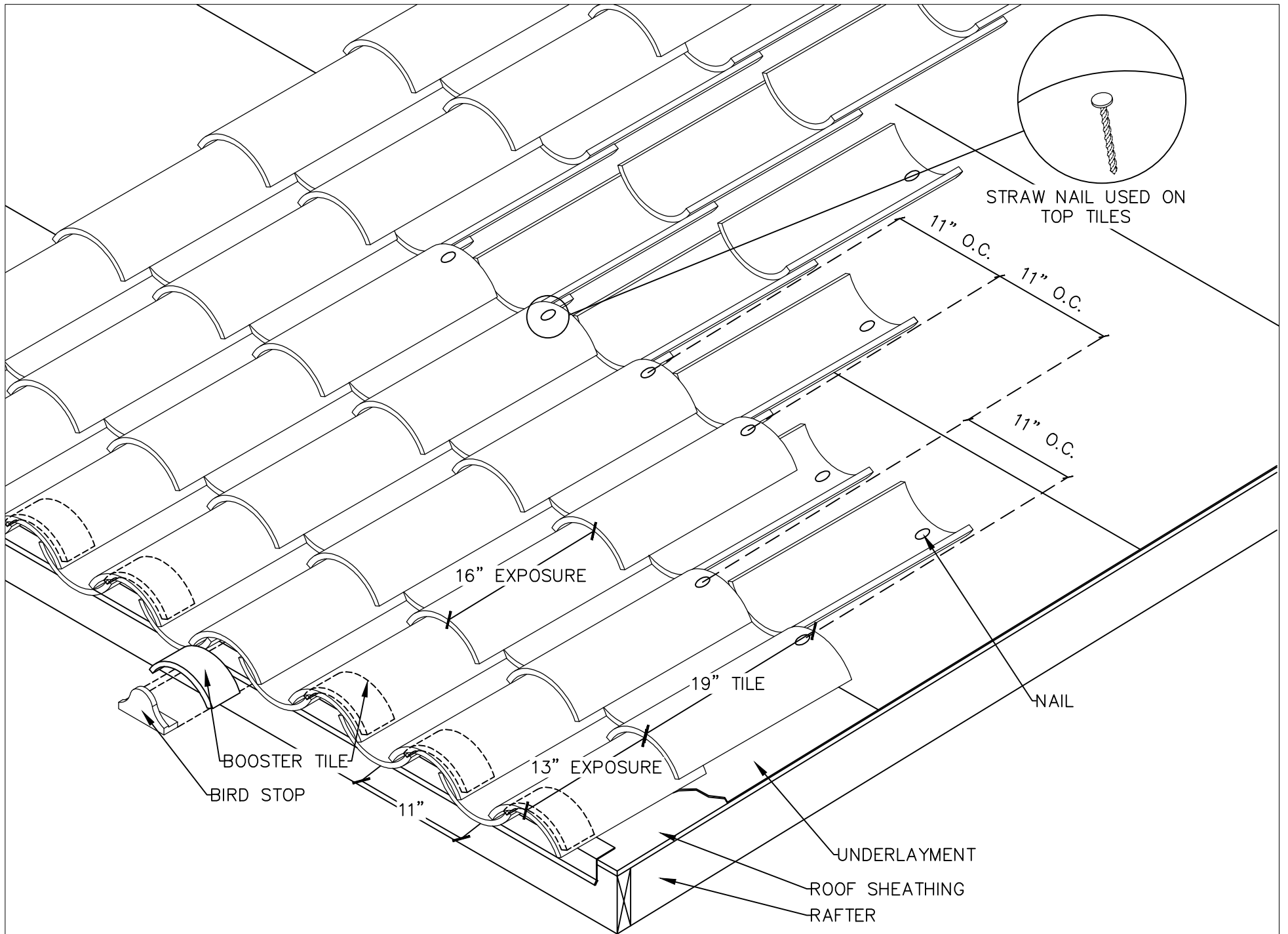
8" STRAIGHT BARREL MISSION NAIL ON SYSTEM
