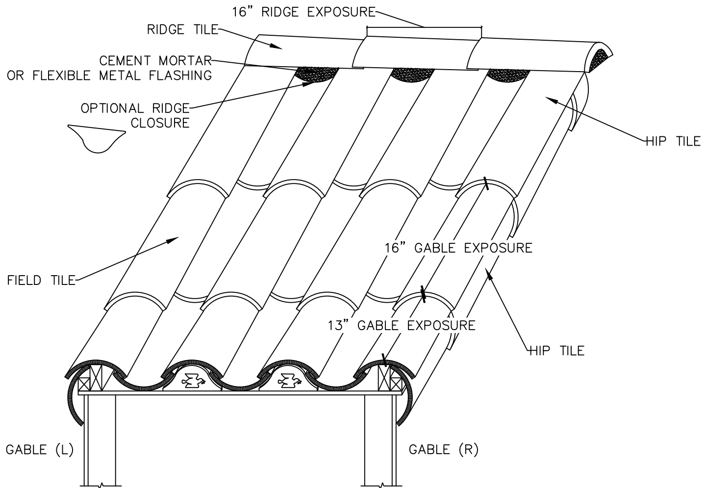
FIELD DETAIL
