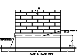
CHIMNEY FLASHING
