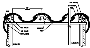
GABLE/EAVE DETAIL
