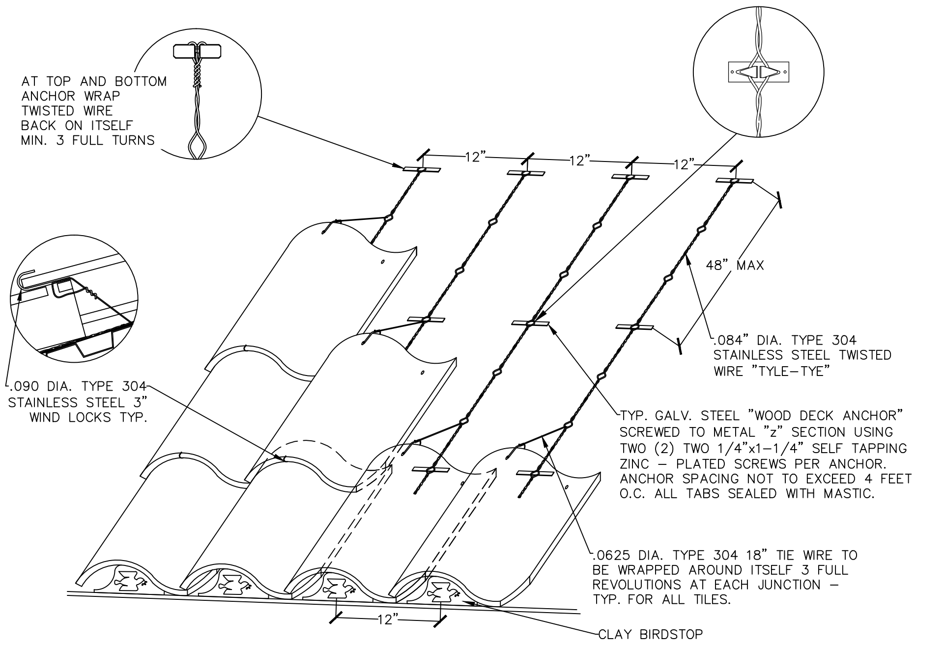
"S" MISSON "TYLE-TYE" FIELD DETAIL (MTL. DECK) MCA - SMISS - MTL - 3D N.T.S.
