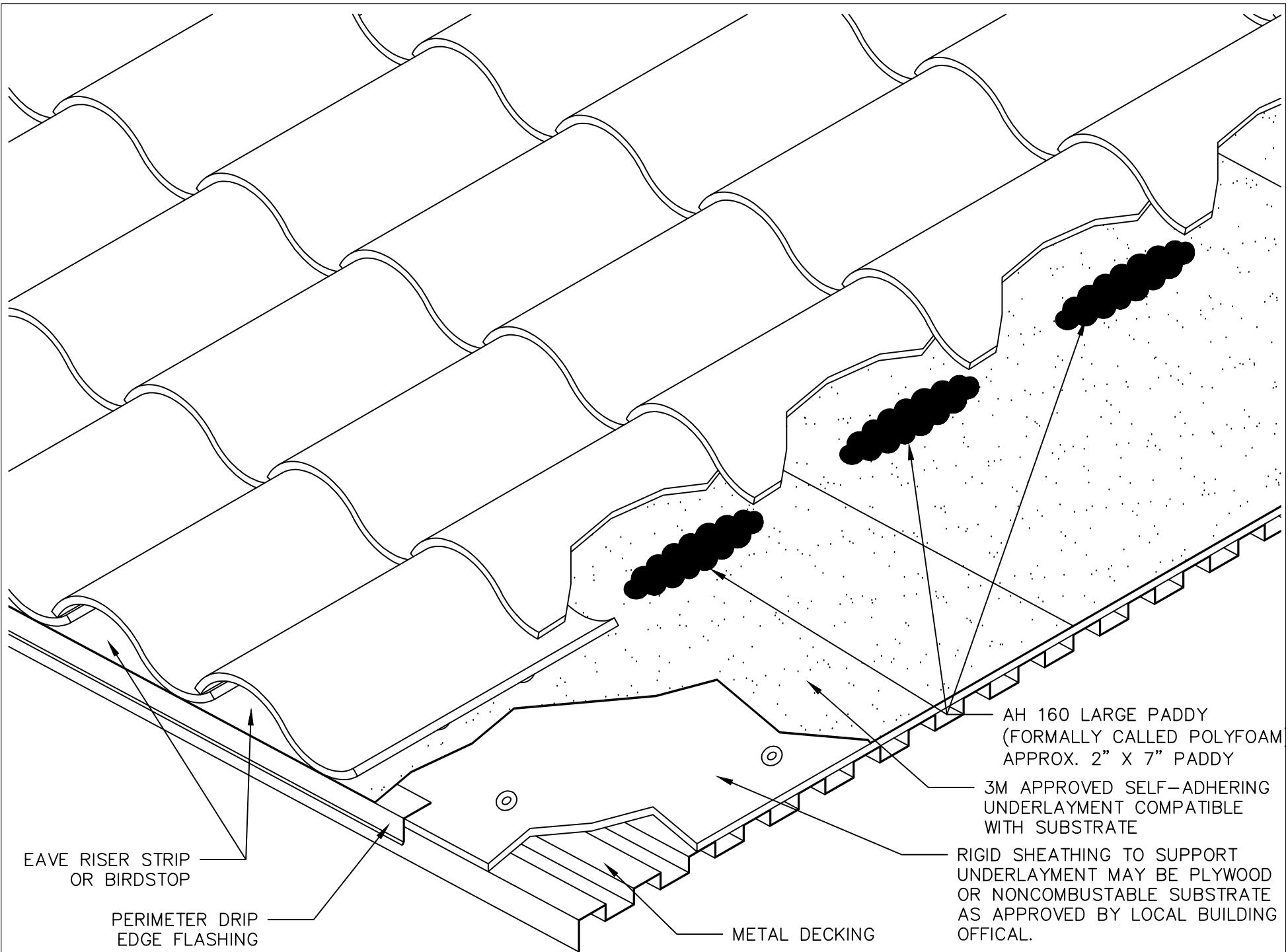
AH 160 (POLYFOAM ADHESIVE) LARGE PADDY APPLICATION
