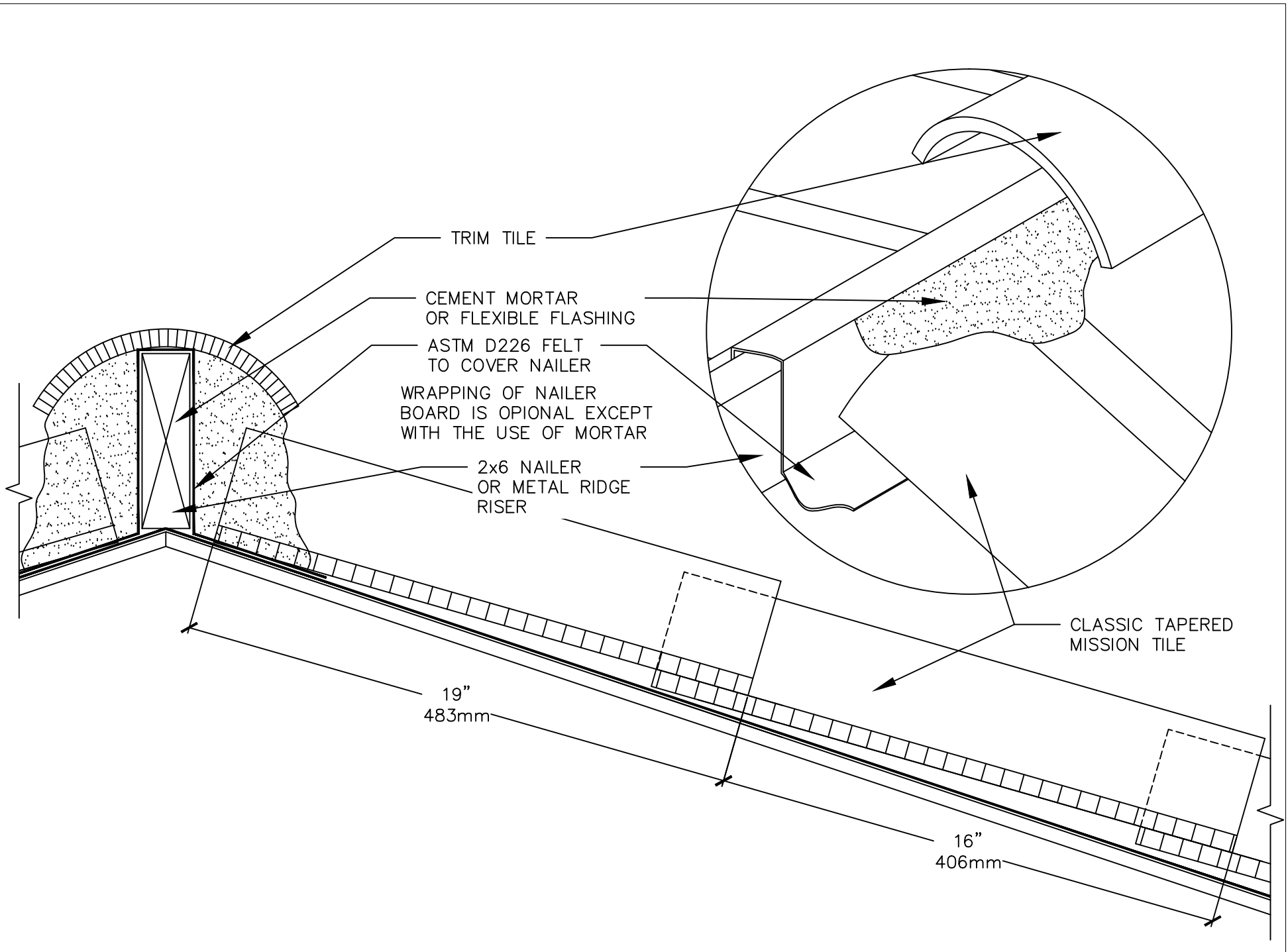
RIDGE & HIP PLATE END DETAIL
