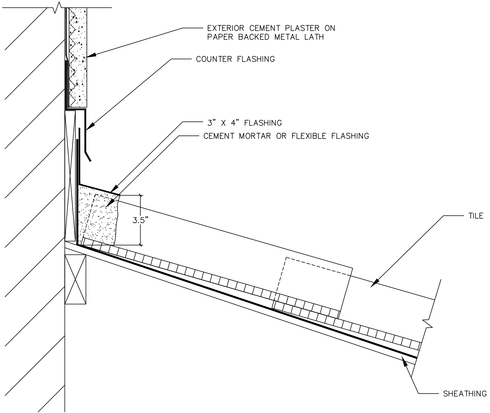
FLASHING AT WALL
