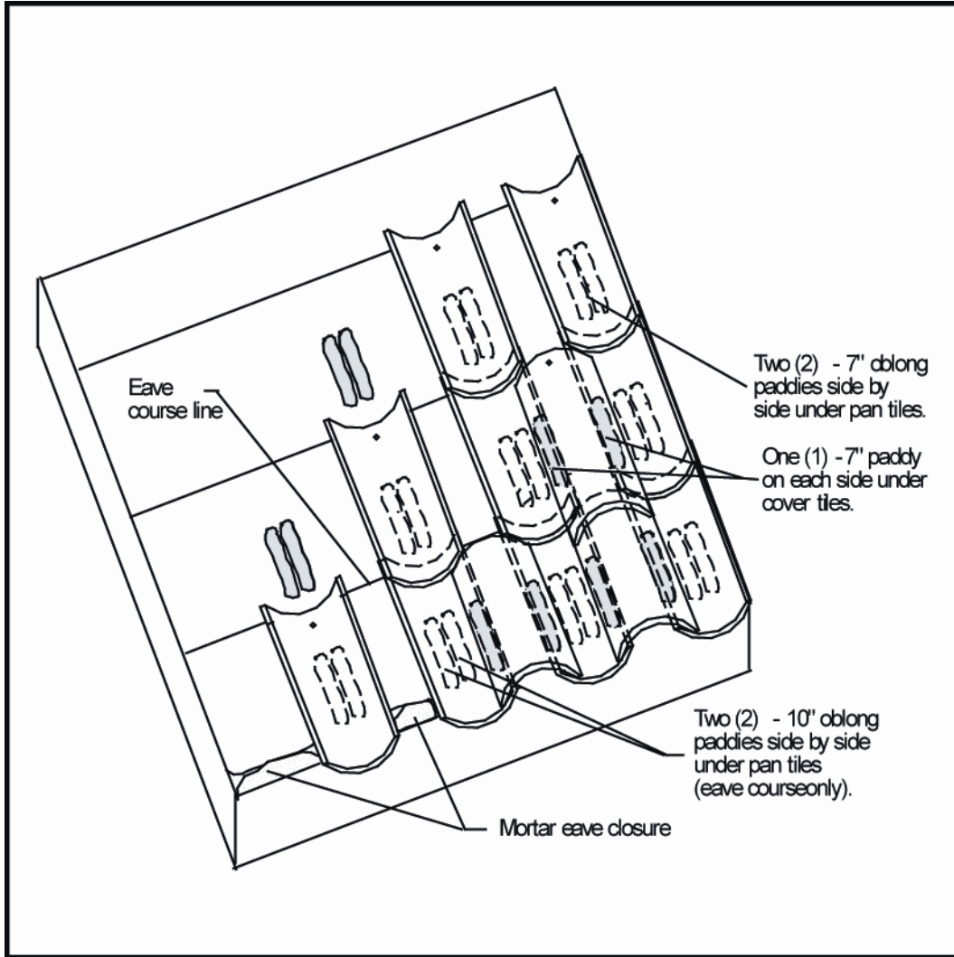
2-PIECE BARREL PROFILE
