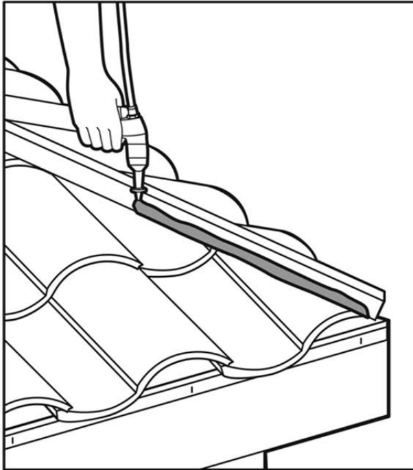
A bead of ICP Polyset®AH-160 may be applied above the field tile surface on both sides of the hip/ridge board or galvanized metal frame to provide weatherblocking.
