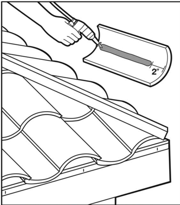
To attach hip/ridge tiles, a bead of ICP Polyset®AH-160 roof tile adhesive may be applied along the full length of the tile excluding 2 inches excluding 2 inches on the eave end of tile.
