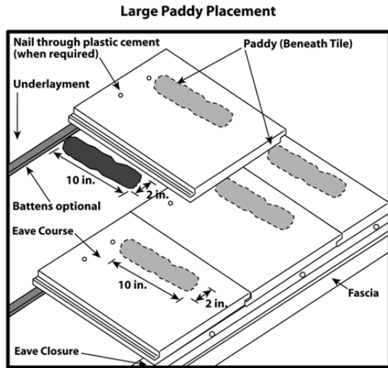
Flat/Low Profile Tile
