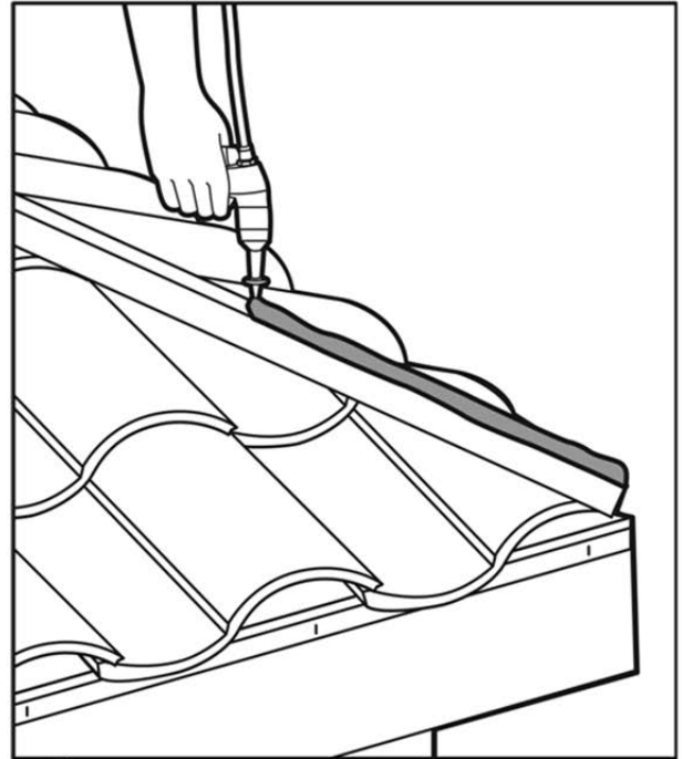
To attach hip/ridge tiles, a bead of ICP Polyset®AH-160 may be applied down the center of the hip/ridge board or galvanized frame.
