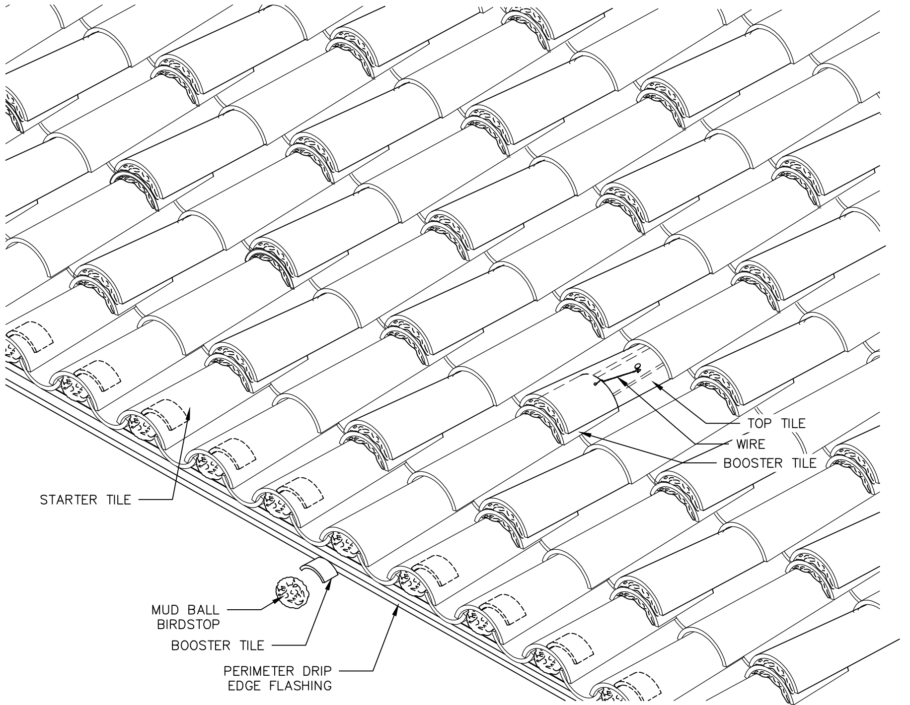
TWO PIECE MISSION MORTAR BOOSTER
